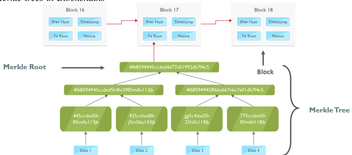
Figure 4 Merkle trees in Blockchains
